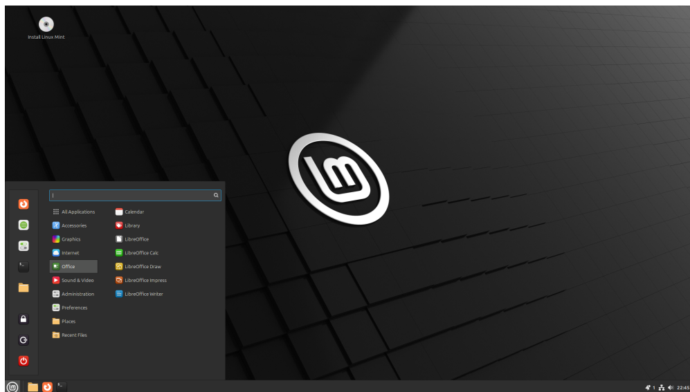
Fig. 1: Cinnamon
